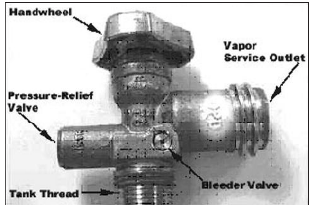
Photo 3: OPD cylinder valve
